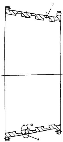
SECTION J-3 (4-7.5H)
