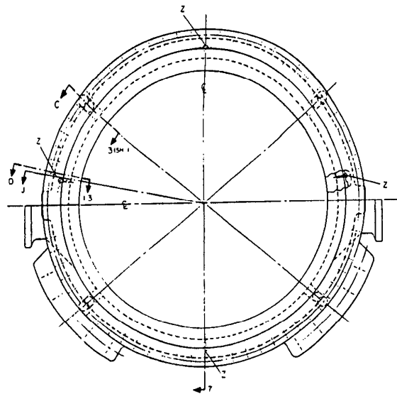
VIEW J-3 (4-7.5H)
