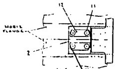
SECTION M-2 (L-11) TOP CROSS SECTION-12 PLACES CHAMFERED 4:1 (12 HOLES, 17) OTHERWISE SAME AS SECT M-7
