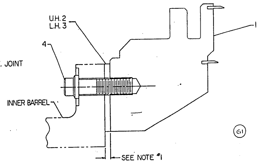
SECTION D-5
